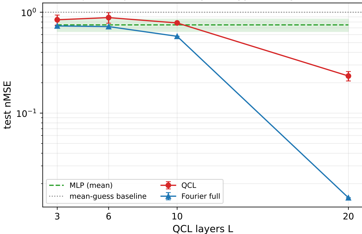
XY quench dynamics — target: staggered magnetization
