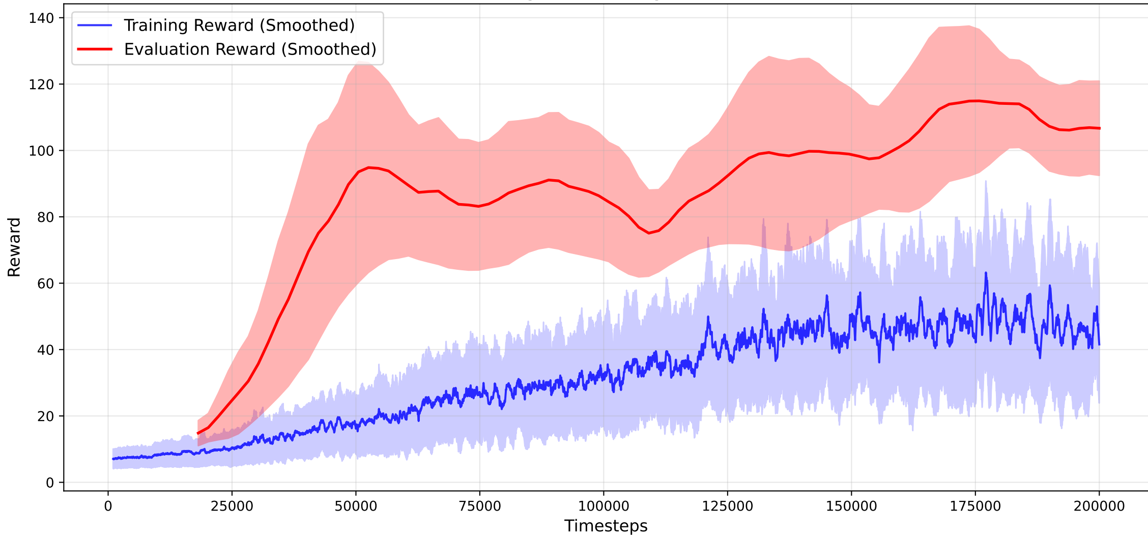
PPO Learning Curve (Avg over 3 seeds)
