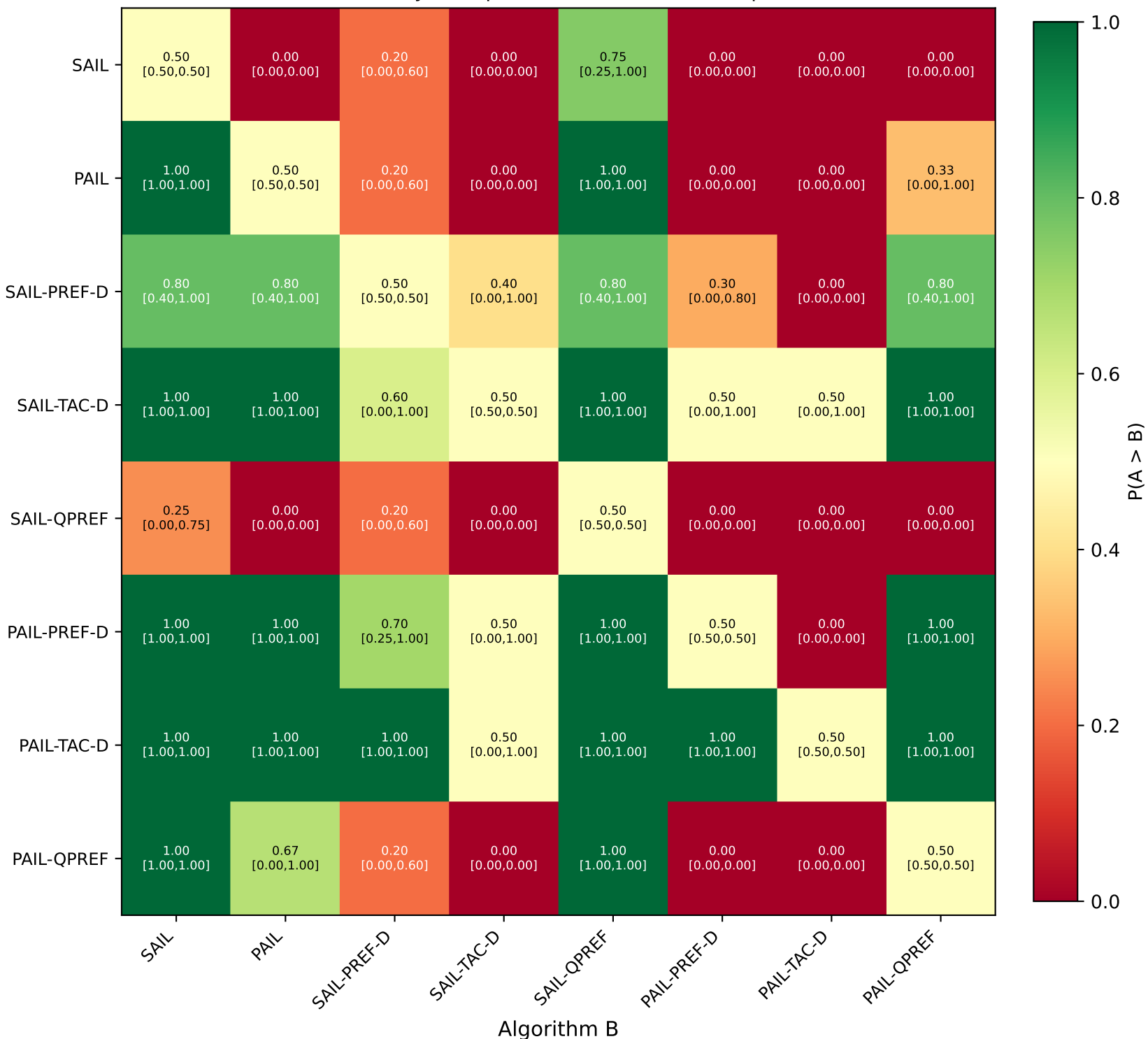
Probability of Improvement (95% Bootstrap CI)
