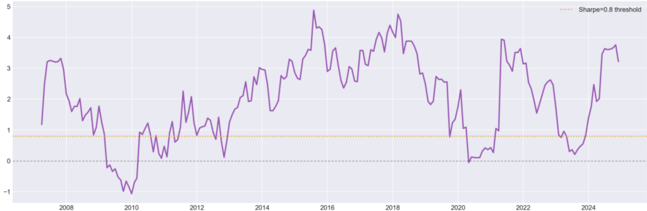
Rolling 12-Month Sharpe — cart
