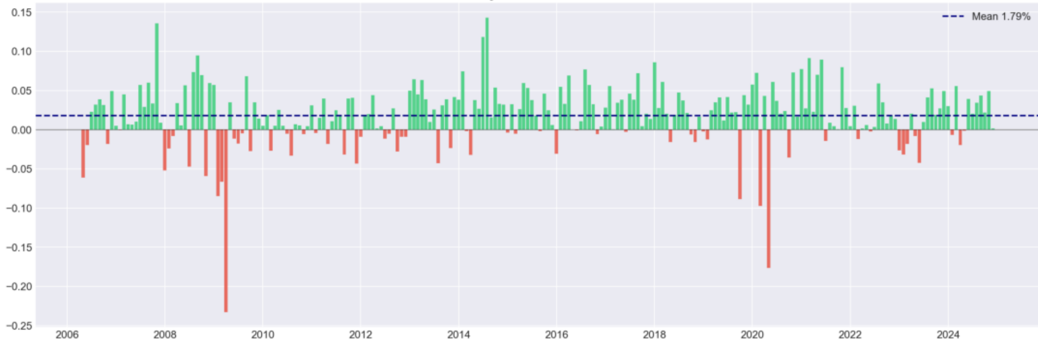
Monthly Net Returns — cart
