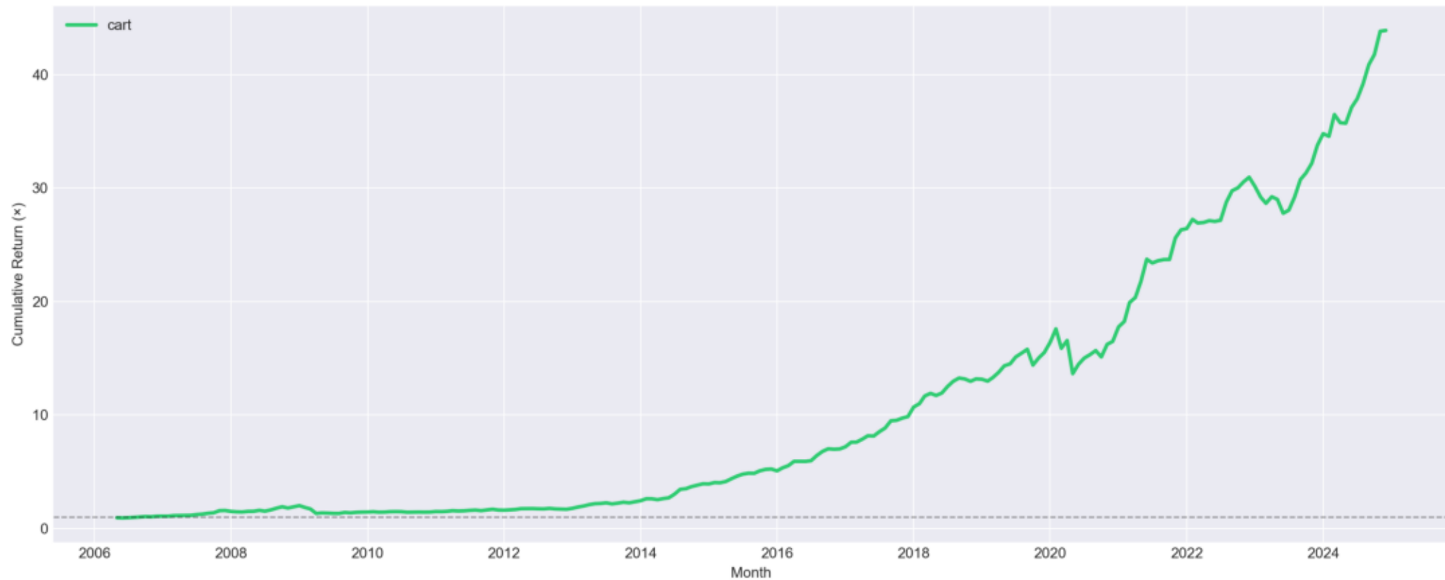
Cumulative Net Return — cart
