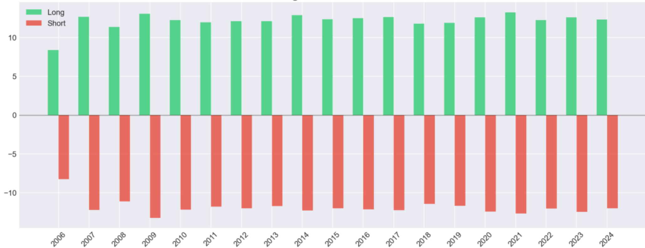
Annual Long/Short Contribution — cart
