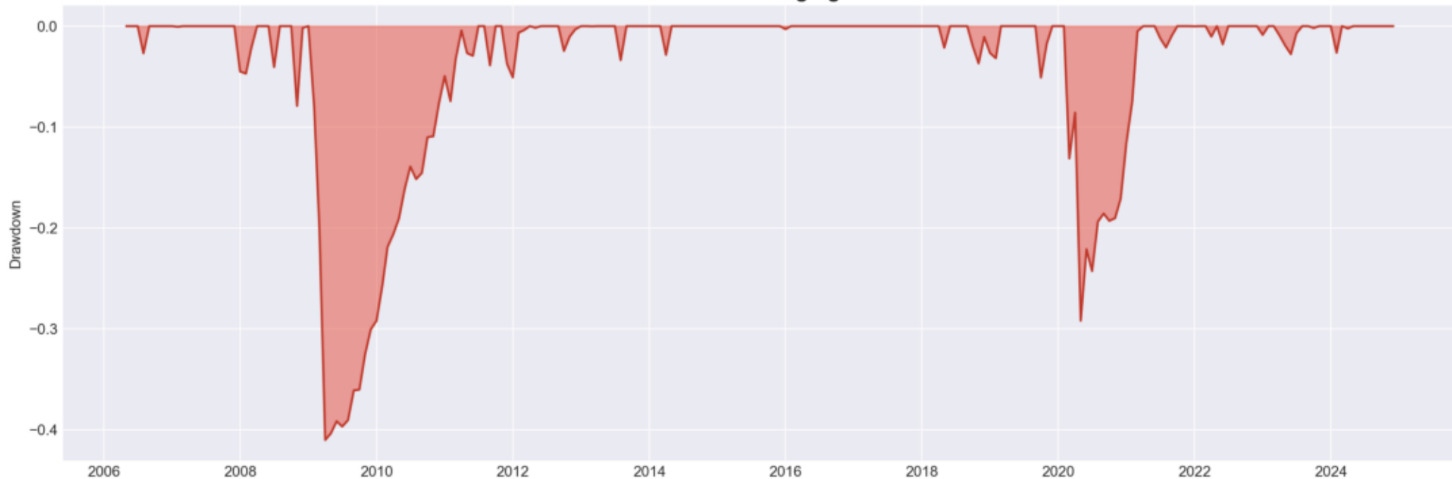
Drawdown — lightgbm
