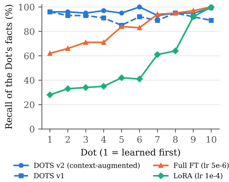
Figure 1: Recall of each Dot’s facts after all ten Dots were learned. Baselines forget earlier chunks; DOTS does not.
