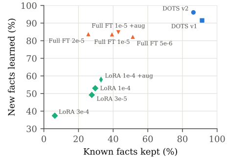
Figure 2: New facts learned against known facts kept, for every run in Table 1.
