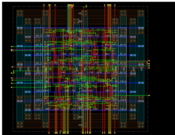
(a) Layout after initial routing, before optimization.
