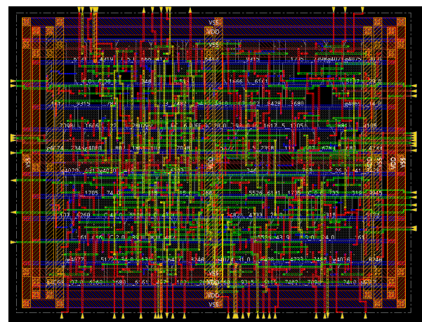
(b) Final layout after post-nano optimization.
