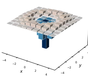
sampled at the pixels: a 9x9 kernel
