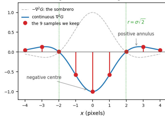
slice through the centre; the weights sum to 0
