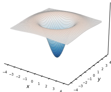
continuous \nabla^2 G(x, y) , \sigma = 1.4
