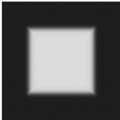
zoomed on a corner: the crossing runs between the pixels, and never breaks
