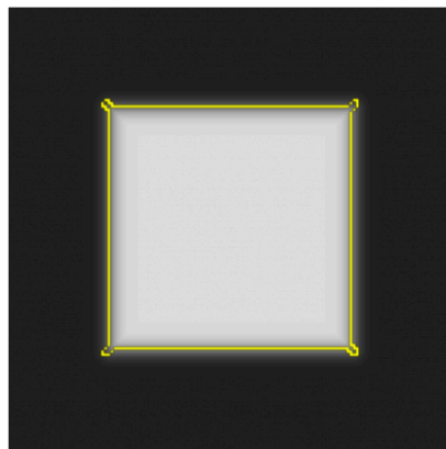
the same curve laid back over f : it traces the boundary
