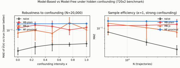
Figure 1. Naive vs. model-based (plain/shrunk) vs. model-free, 5-seed 95% CIs. Left: vs. confounding strength \kappa at N=20,000 . Right: vs. sample size at \kappa=1 . Naive stays lowest throughout.
