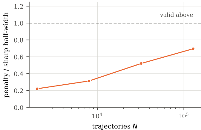
(b) does it cover the identified set?
