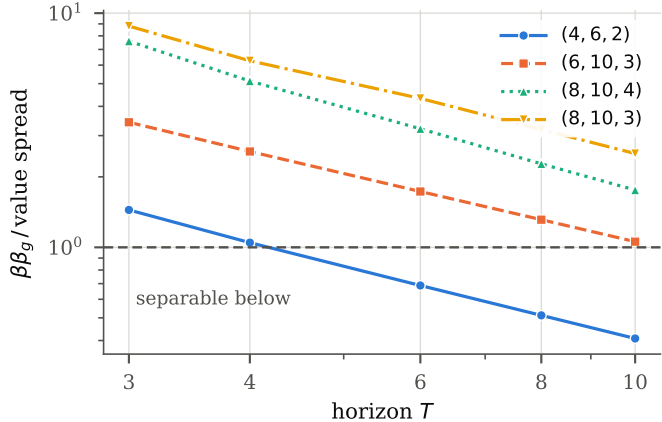
(a) can any valid region order the policies?
