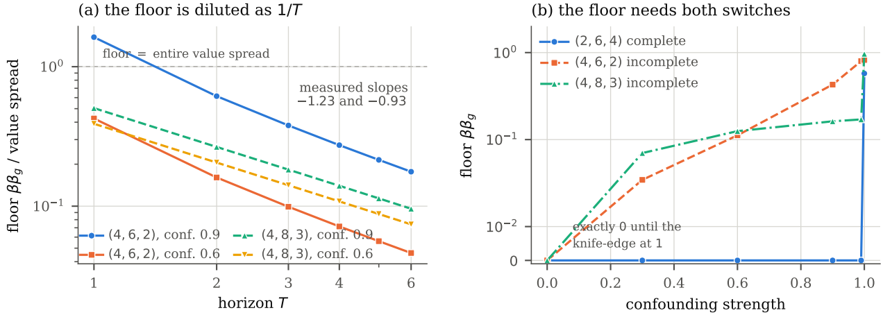
Figure 1. (a) The floor divided by the spread of true values over six candidate policies, against horizon, on log-log axes. Four configurations lie on near-parallel lines with measured exponents -1.23 and -0.93 . At T=1 under strong confounding the floor exceeds the entire spread, so pessimism cannot discriminate at all. (b) The floor against confounding strength. The complete design is at exactly zero until the knife-edge at 1, while the incomplete ones rise smoothly — the conjunction of Corollary 3 seen directly. Zeros are plotted at zero on a symlog axis rather than clamped onto a log decade. Numbers in Appendix D.
