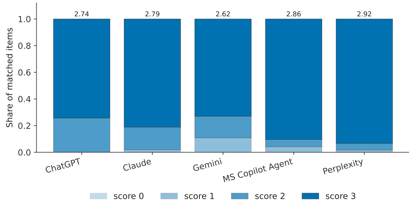
Specificity of matched items (substitute for citation validity)
