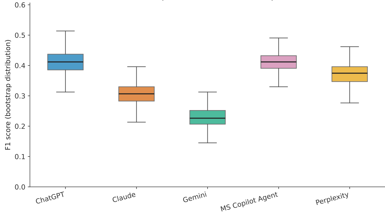
F1 score by system — CEO task (bootstrap distribution, 1000 resamples)
