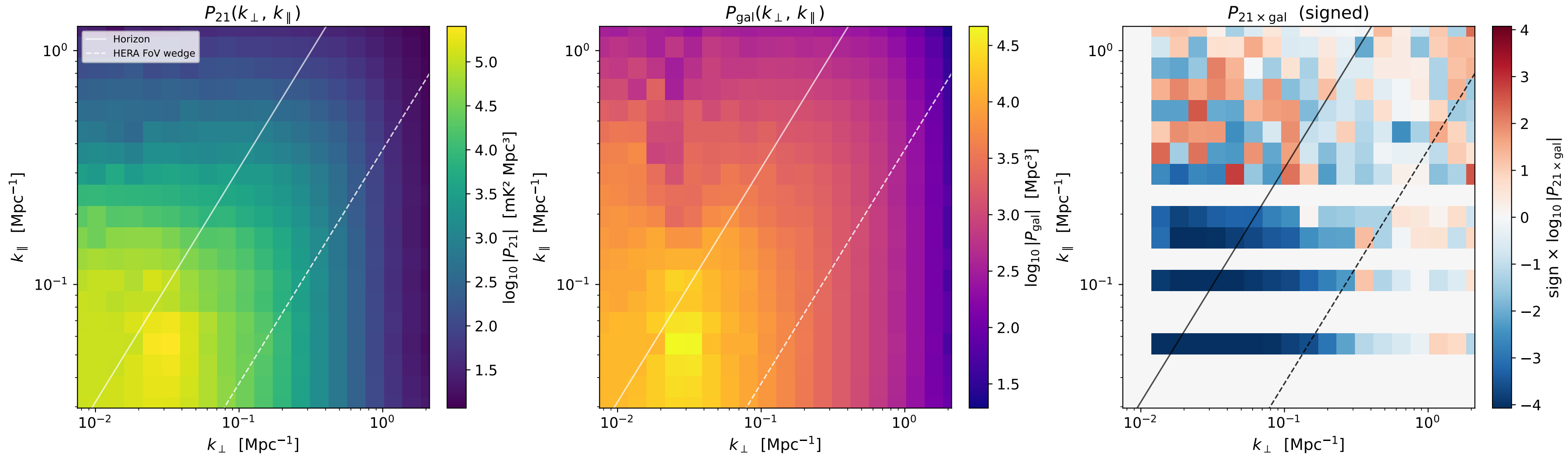
2D cylindrical power spectra — lightcone z = 6.5\text{--}7.5 ( \langle x_{\text{HI}} \rangle = 0.16 , Euclid M_{\text{UV}} < -22 )
