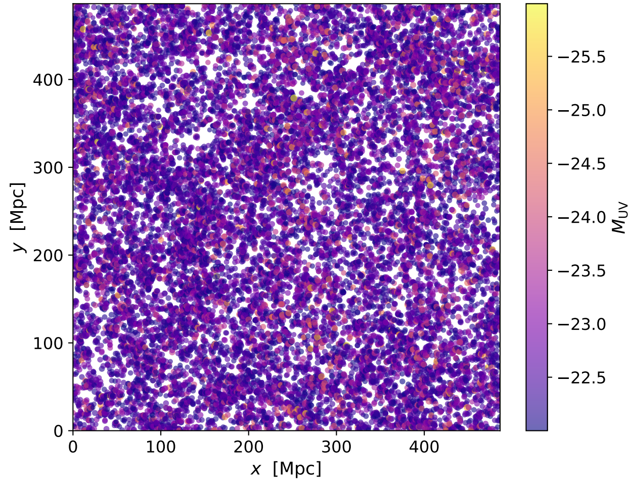
Selected galaxies — projected positions
