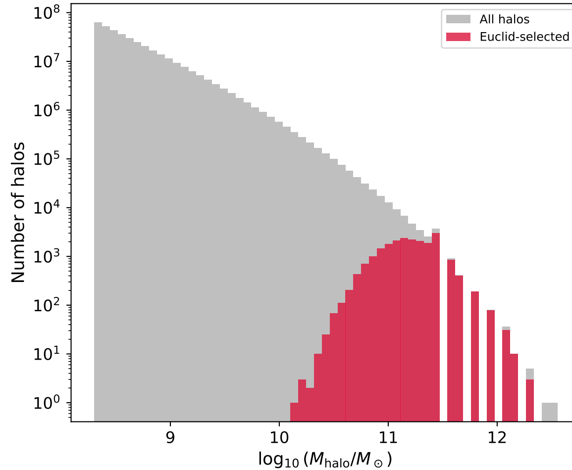
Halo mass — before and after the cut
