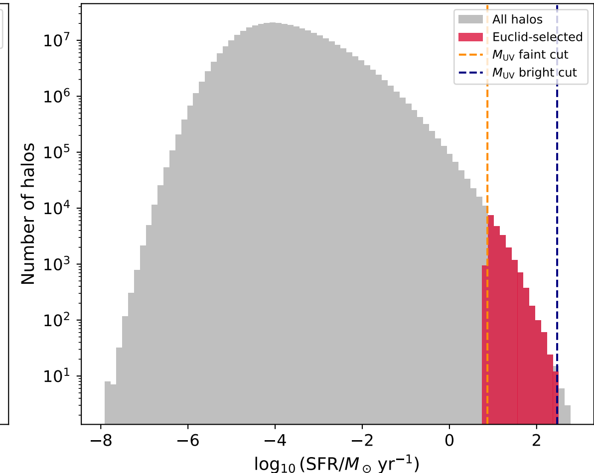
SFR — before and after the cut
