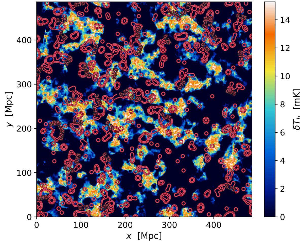
\delta_{\text{gal}} contours over \delta T_b
