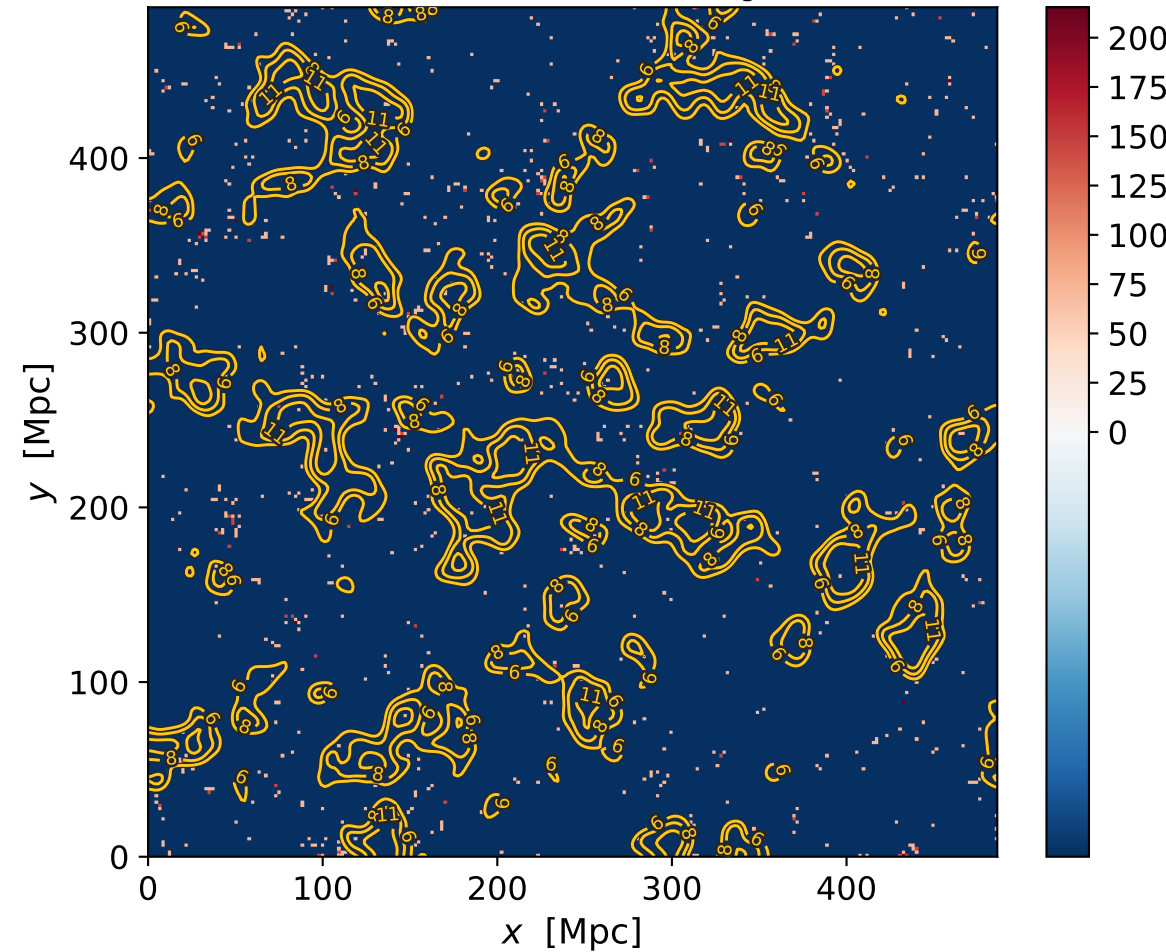
\delta T_b contours over \delta_{\text{gal}}
