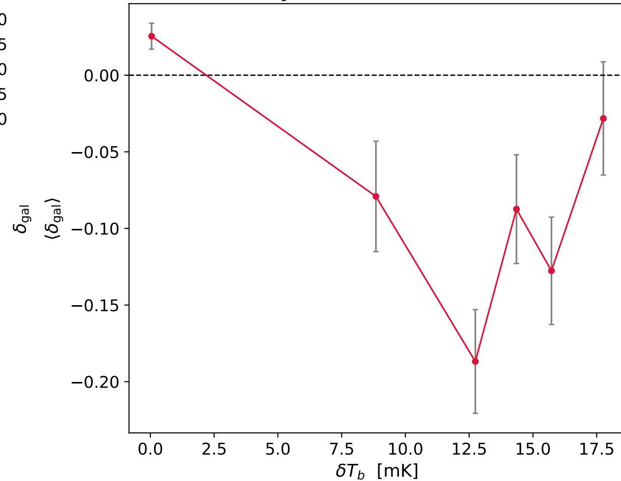
Mean \delta_{\text{gal}} per \delta T_b bin ( r = -0.002 )
