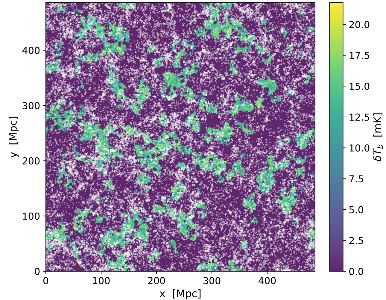
Halos over 21 cm slice at z = 7.0
