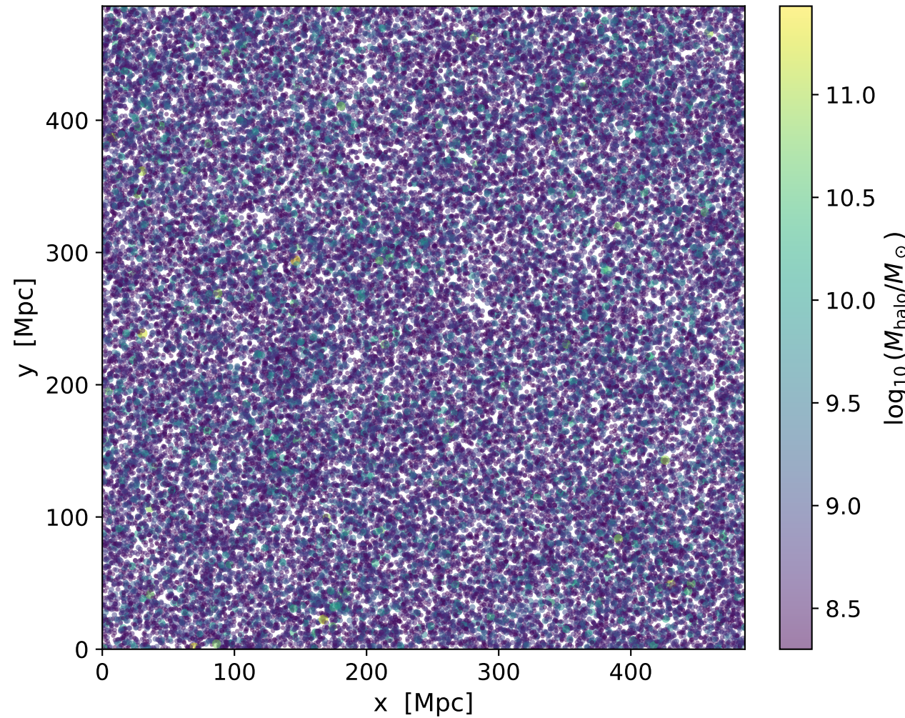
Projected halo catalogue at z = 7.0
