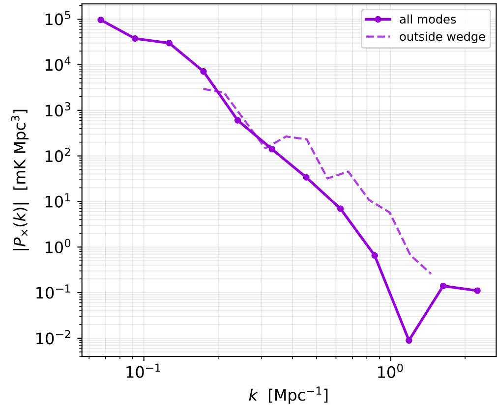
21 cm \times galaxy (negative on large scales; |P_{\times}| shown)
