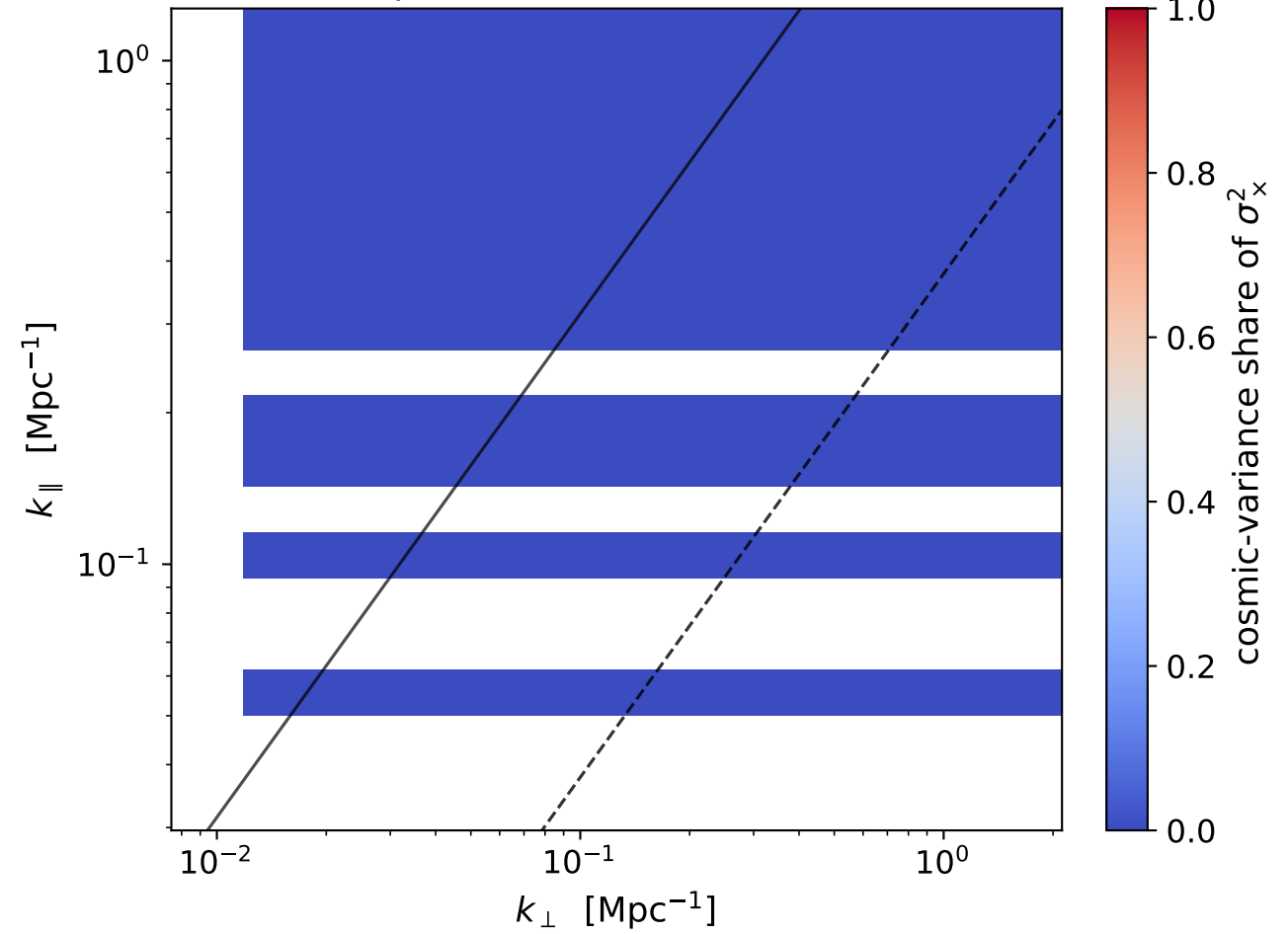
Sample variance (1) vs noise (0)
