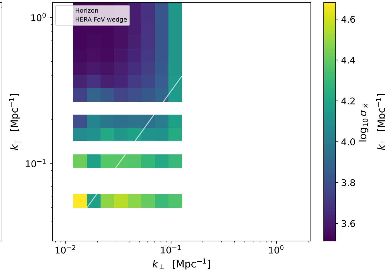
Cross-power uncertainty \sigma_x
