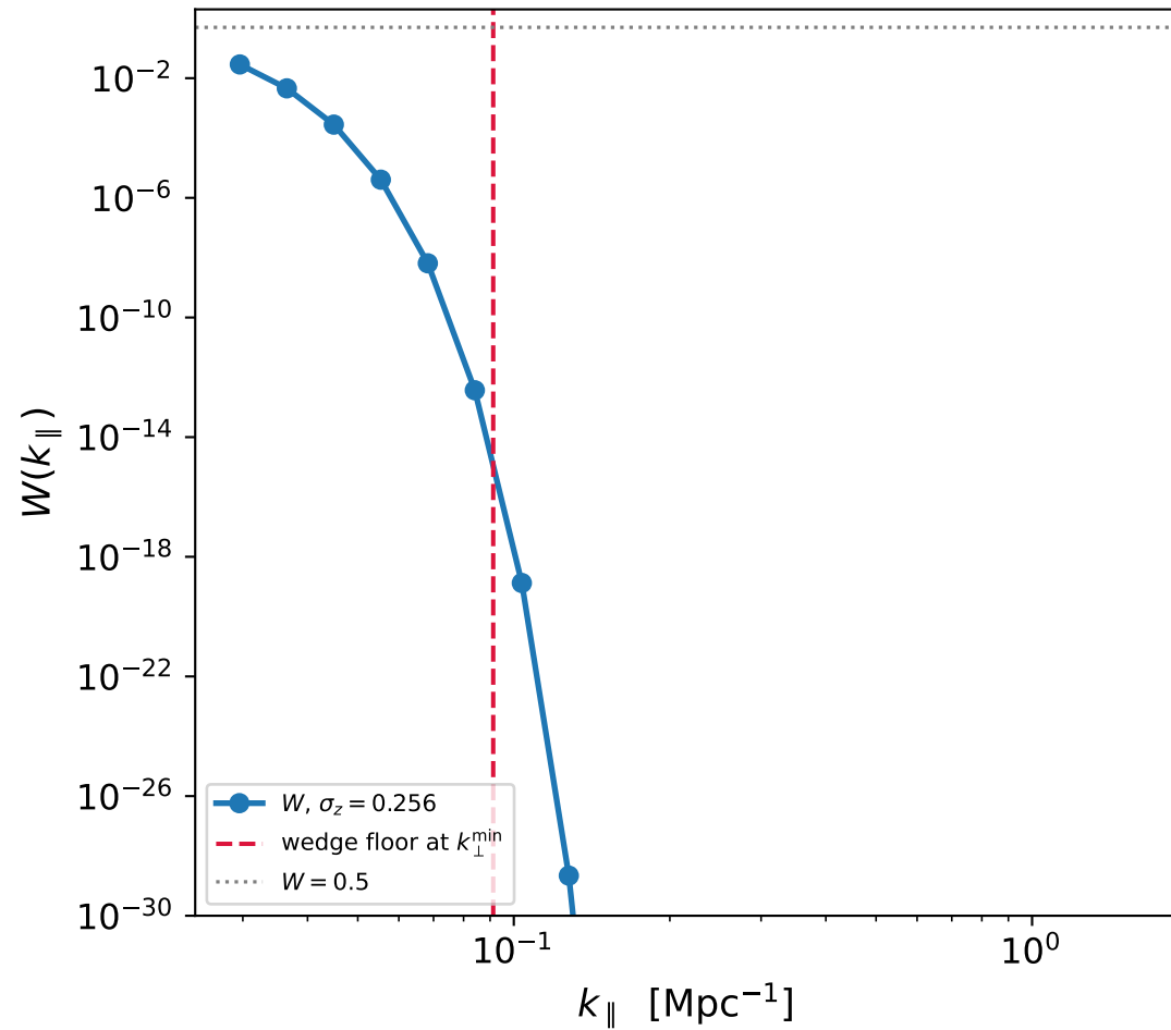
Photo-z damping ( \sigma_r = 90.0 \text{ Mpc} )
