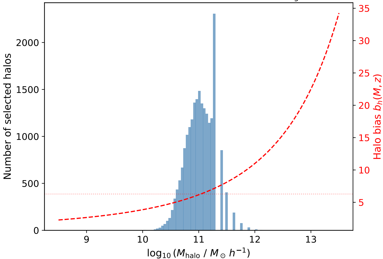
Euclid-selected halos and bias at z = 7.0 ( \langle b_g \rangle = 6.28 )
