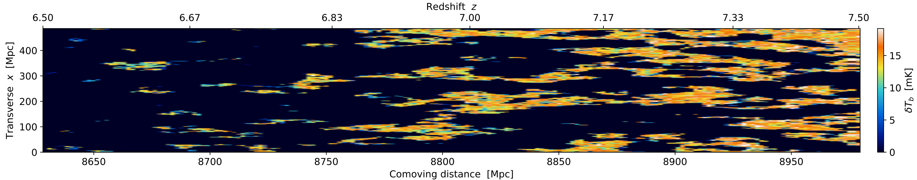
21 cm brightness temperature lightcone slice ( z = 6.5\text{--}7.5 , f_{\text{obs}} = 167\text{--}189 MHz, \langle x_{\text{HI}} \rangle = 0.16 )
