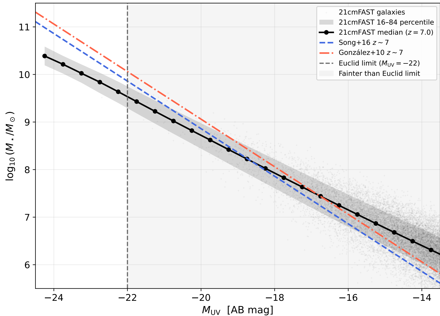
Stellar mass-UV magnitude relation ( z = 7.0 )
