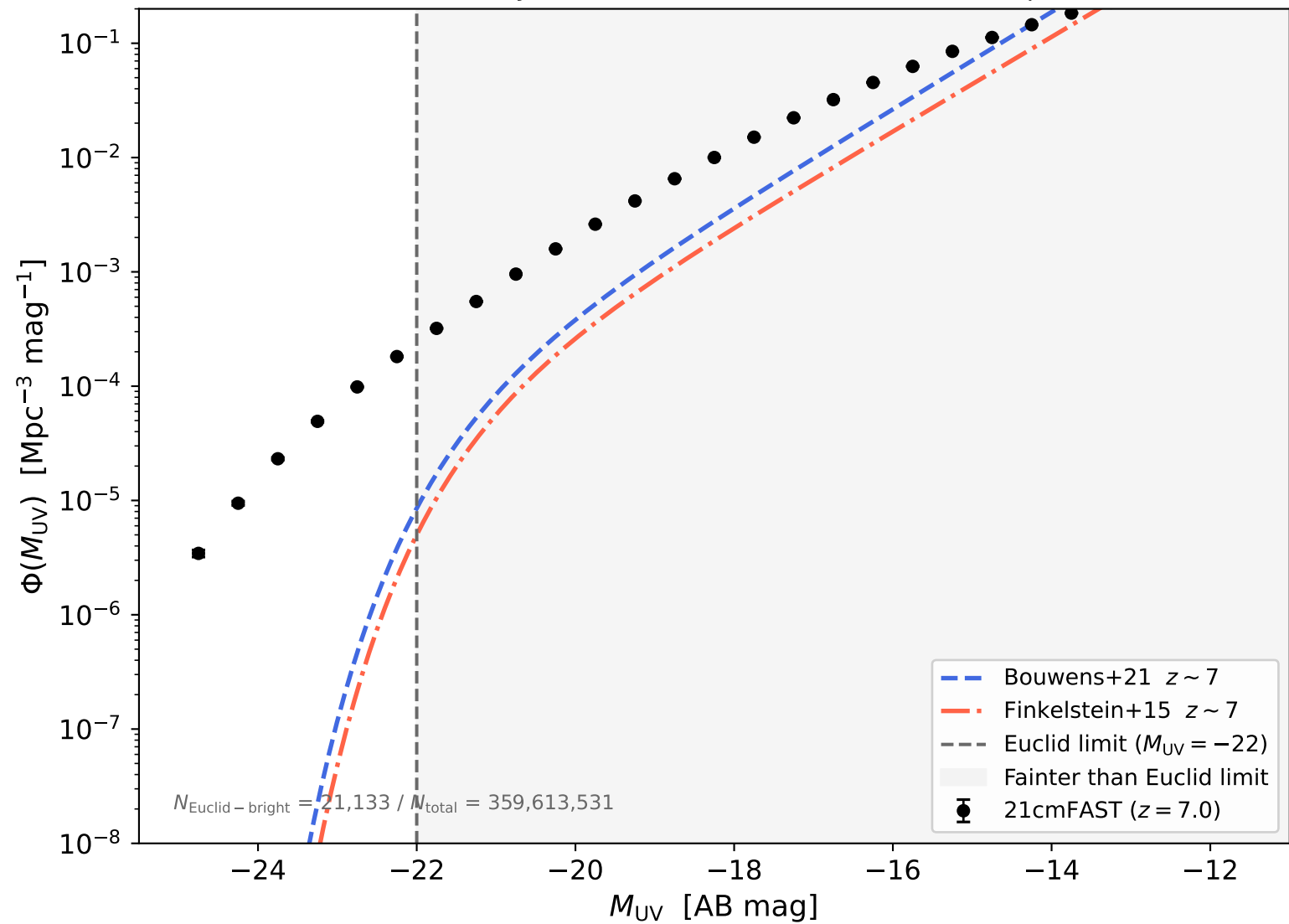
UV luminosity function ( z = 7.0 , V_{\text{box}} = 1.2e + 08 \text{ Mpc}^3 )
