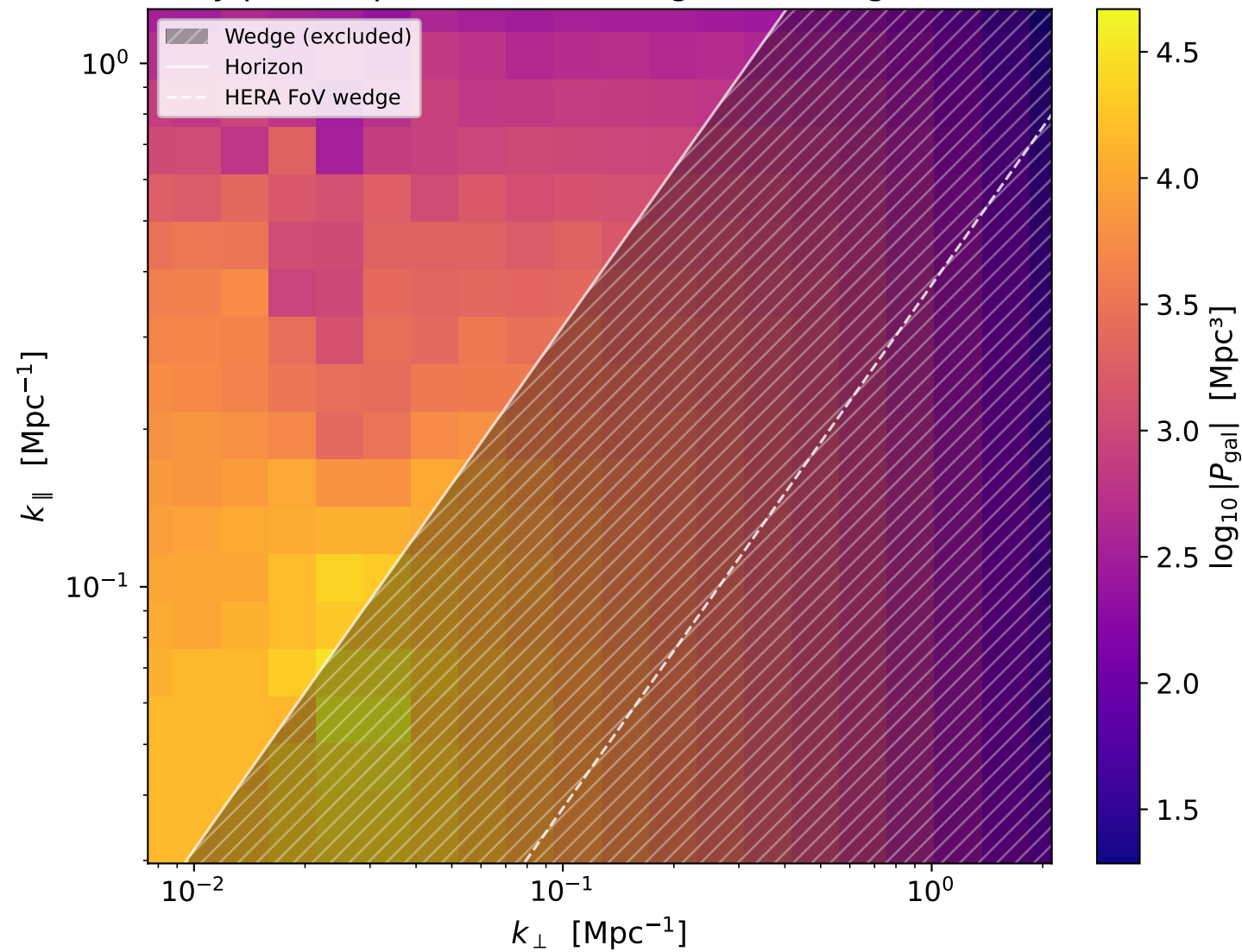
Galaxy power spectrum with foreground wedge, z_{\text{obs}} = 7.0
