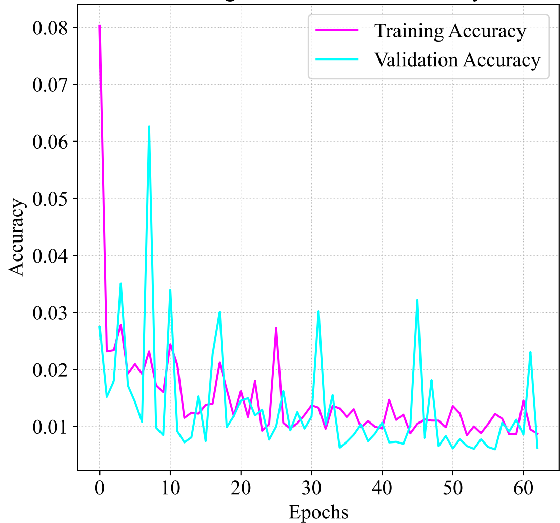
Training and Validation Accuracy
