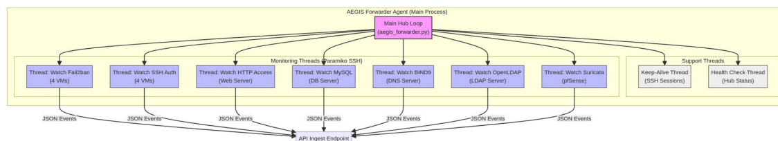
Figure 4.7: AEGIS Forwarder Agent Thread Architecture
