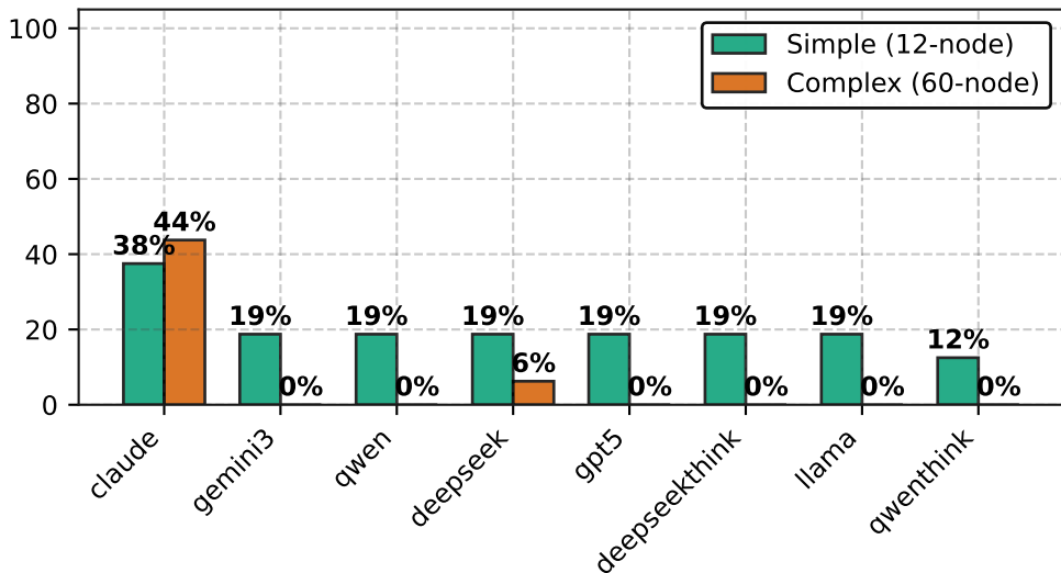
Scalability: LLM Performance on Graph Complexity
