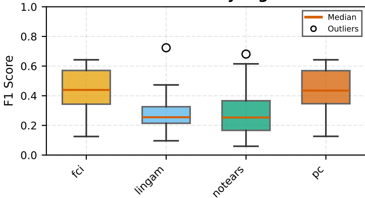
F1 Distribution by Algorithm
