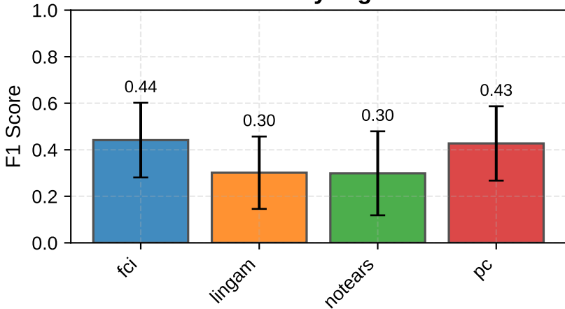
F1 Score by Algorithm
