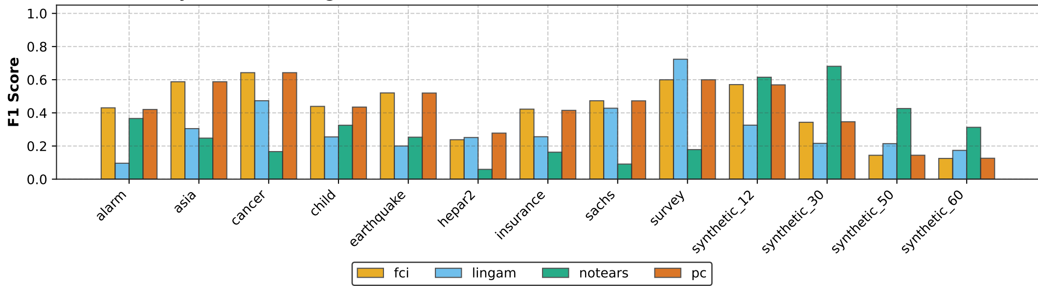
(c) F1 Score by Dataset and Algorithm
