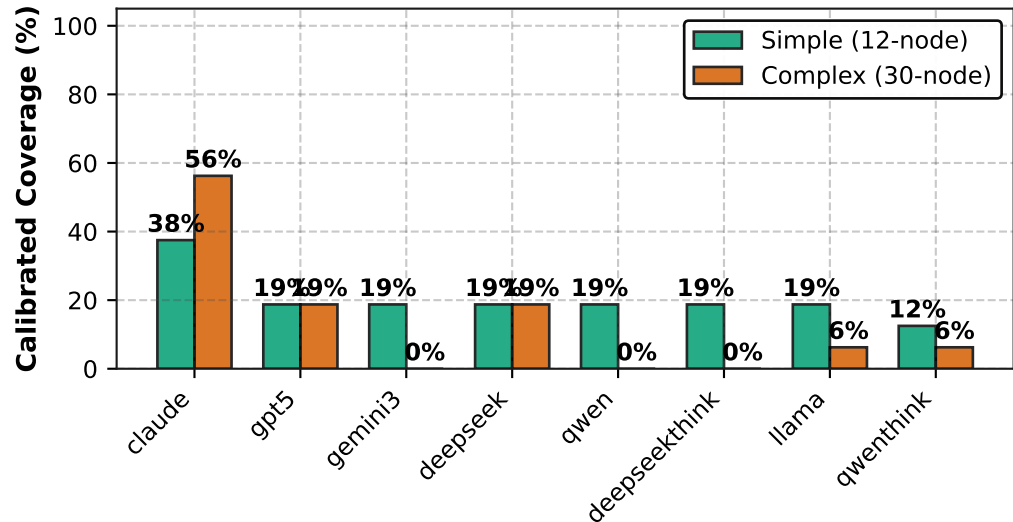
Scalability: LLM Performance on Graph Complexity
