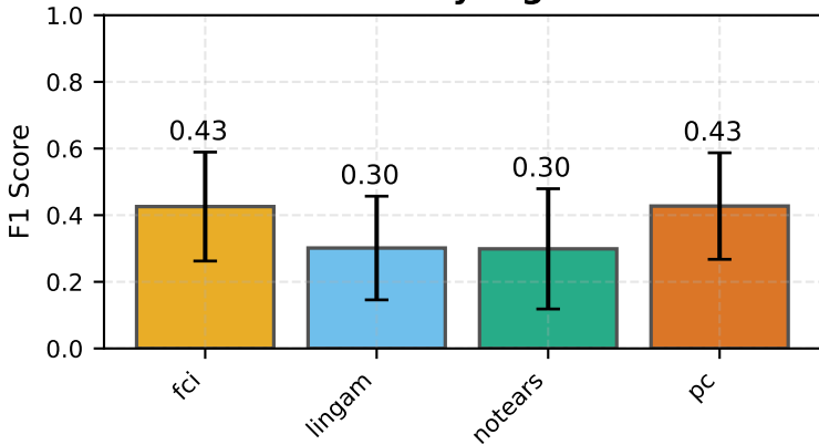
F1 Score by Algorithm
