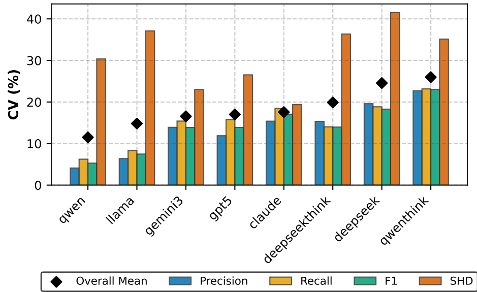
Prompt Robustness: Coefficient of Variation by Model
