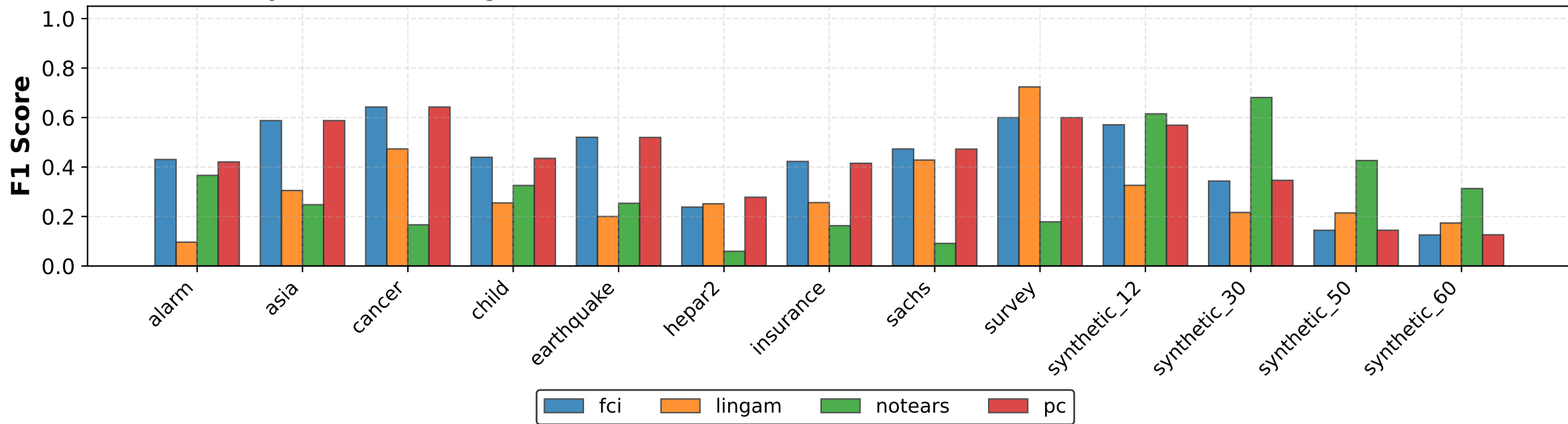
(c) F1 Score by Dataset and Algorithm
