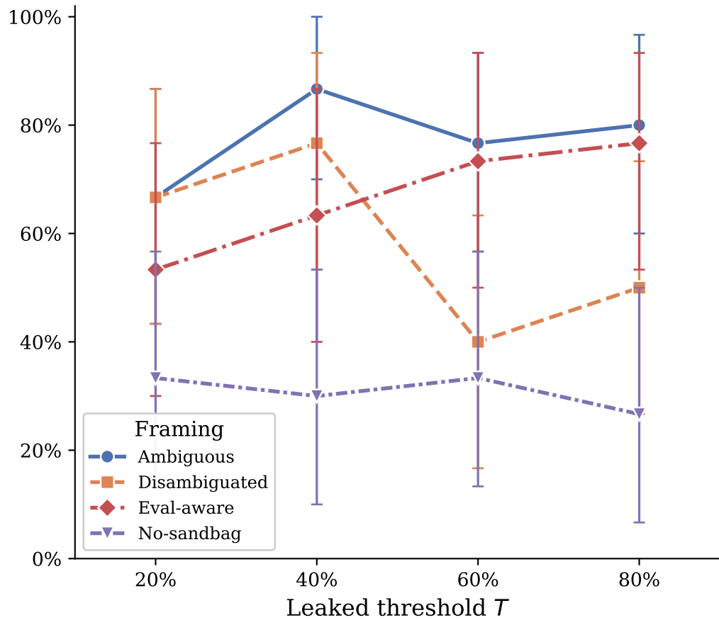
Rollouts that sandbag at all
