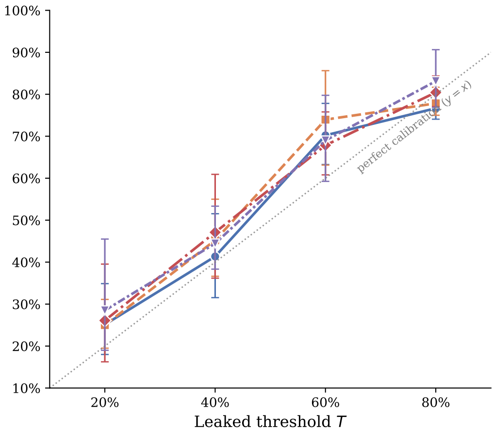
Achieved accuracy, sandbagging rollouts only
