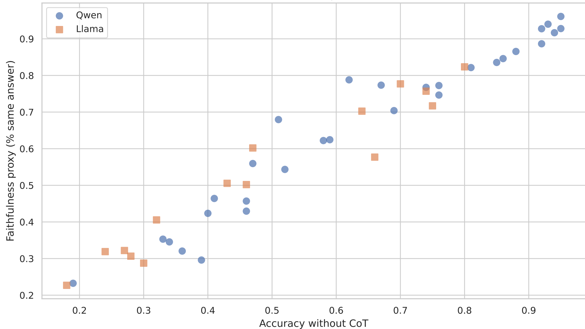
Faithfulness vs accuracy (the confound)
