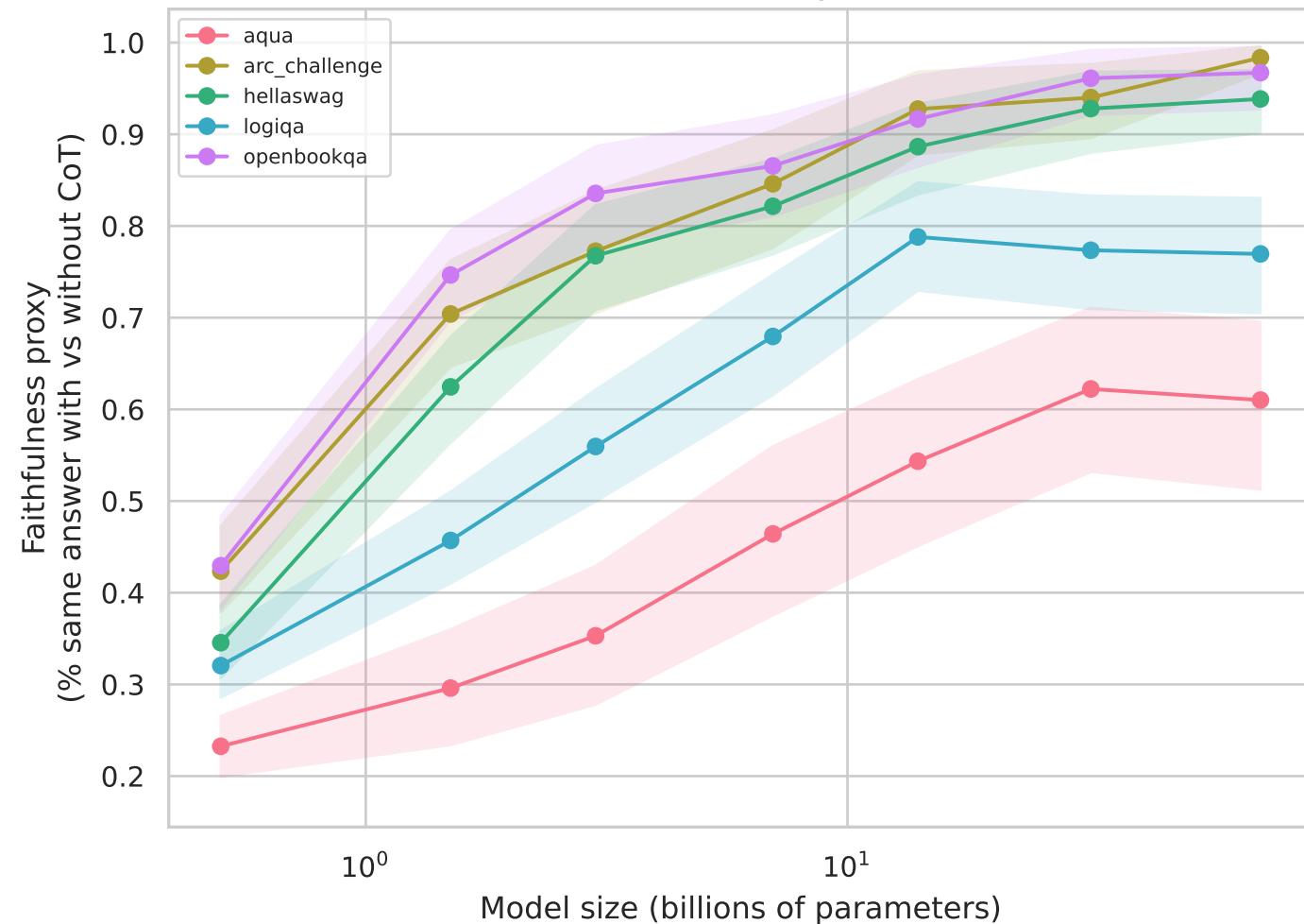
Qwen family
