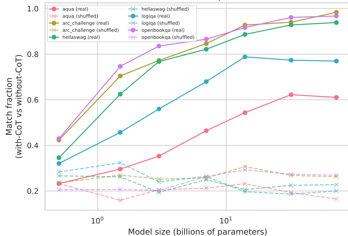
Qwen family
