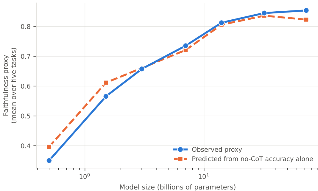
Qwen2.5-Instruct
