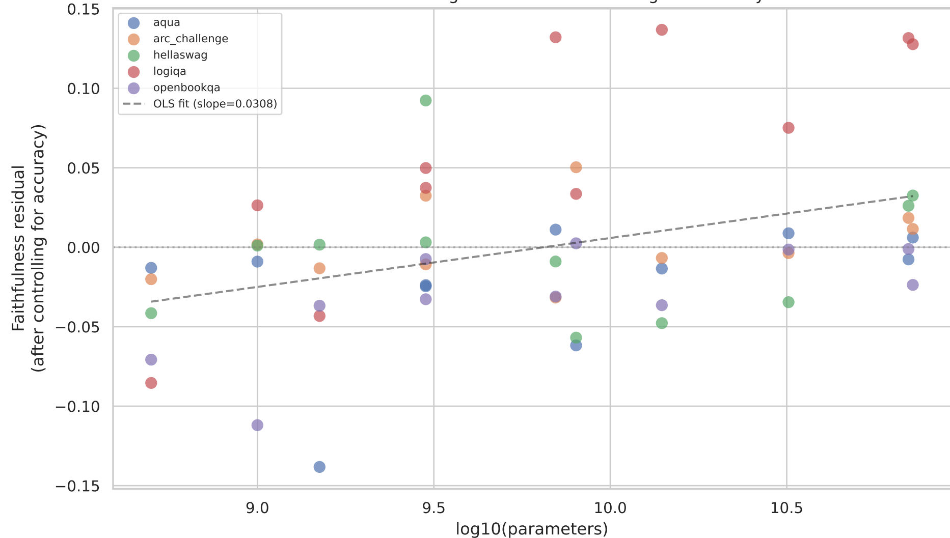
Does inverse scaling survive after controlling for accuracy?
