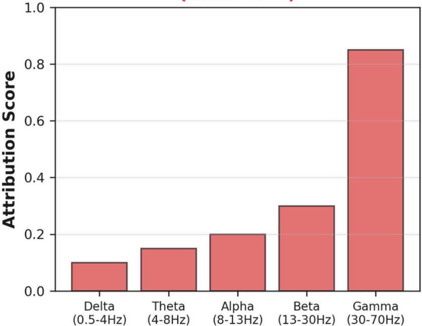
A) Seizure Detection (Conf: 92%)
