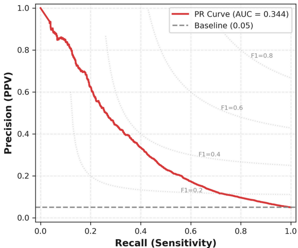
(c) Precision-Recall Curve
