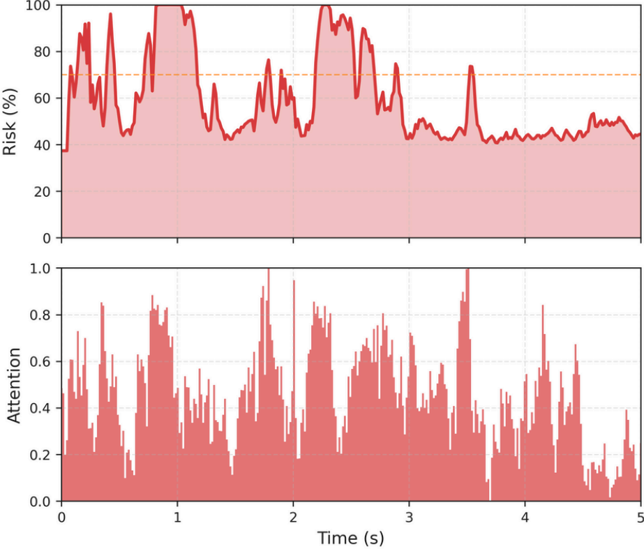
Seizure Sample Mean Risk: 59%
