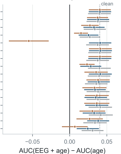
b Increment over age
