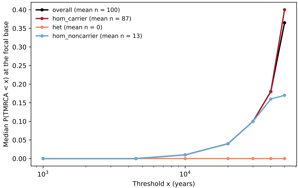
EAS (PHLASH median, custom demography) — descriptive carrier stratification (not the test)
