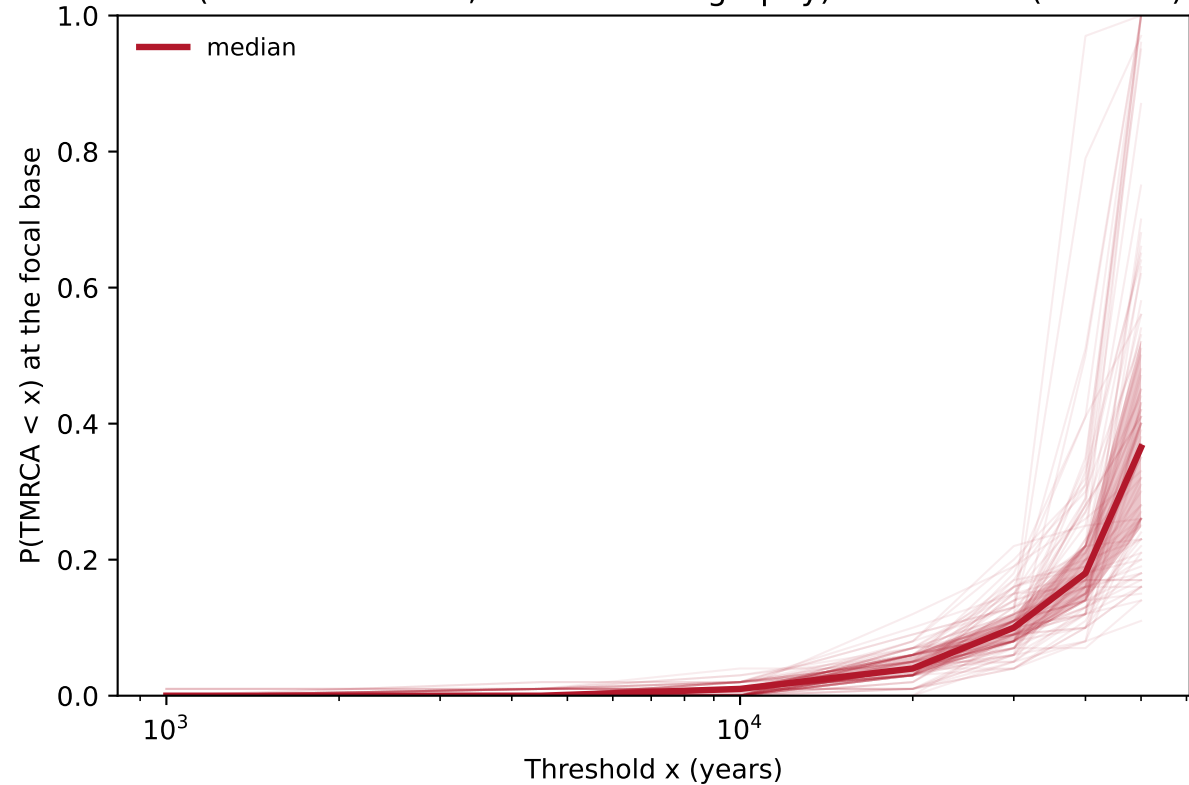
EAS (PHLASH median, custom demography) — selected (n = 100)
