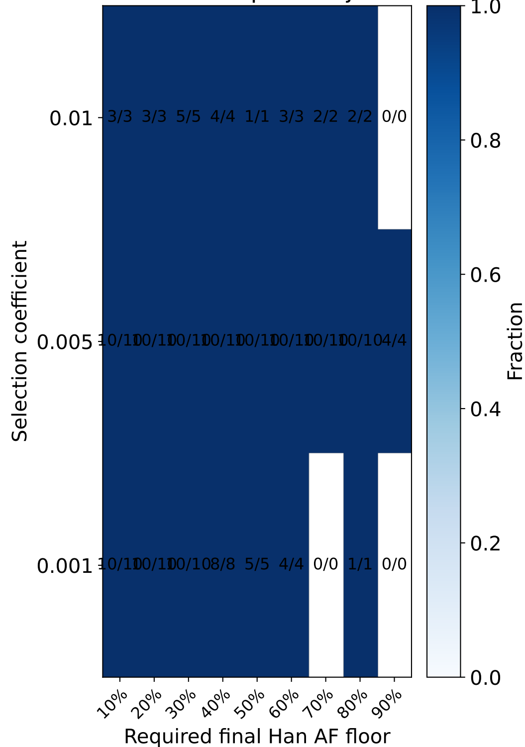
Decoded / accepted trajectories
