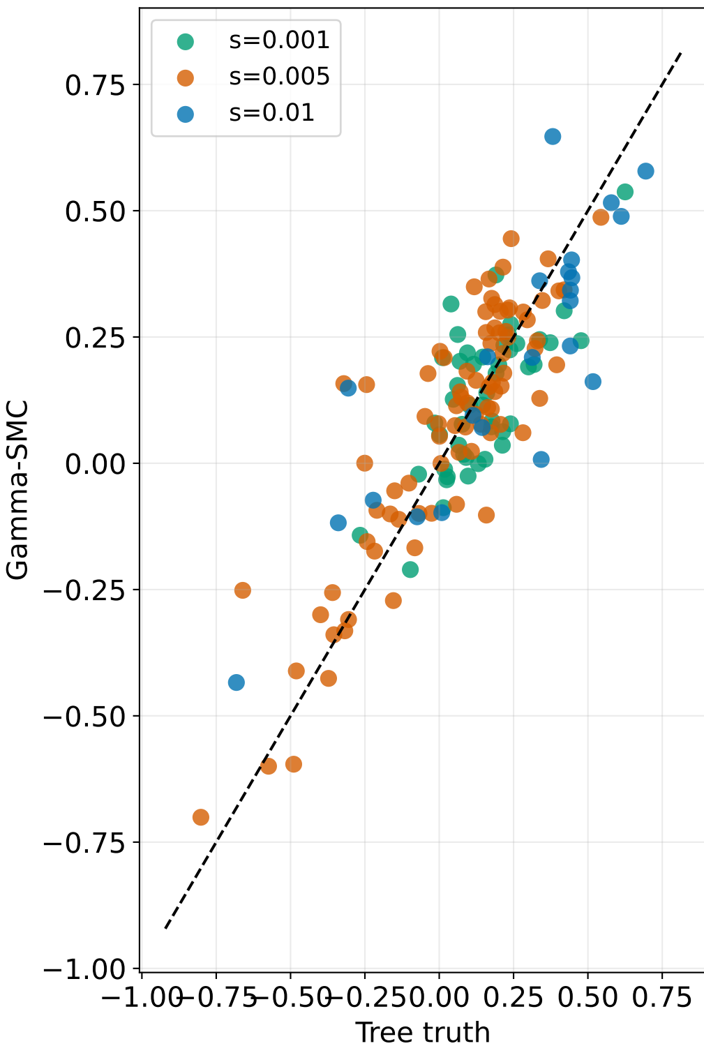
Alt-ref normalized CDF area
