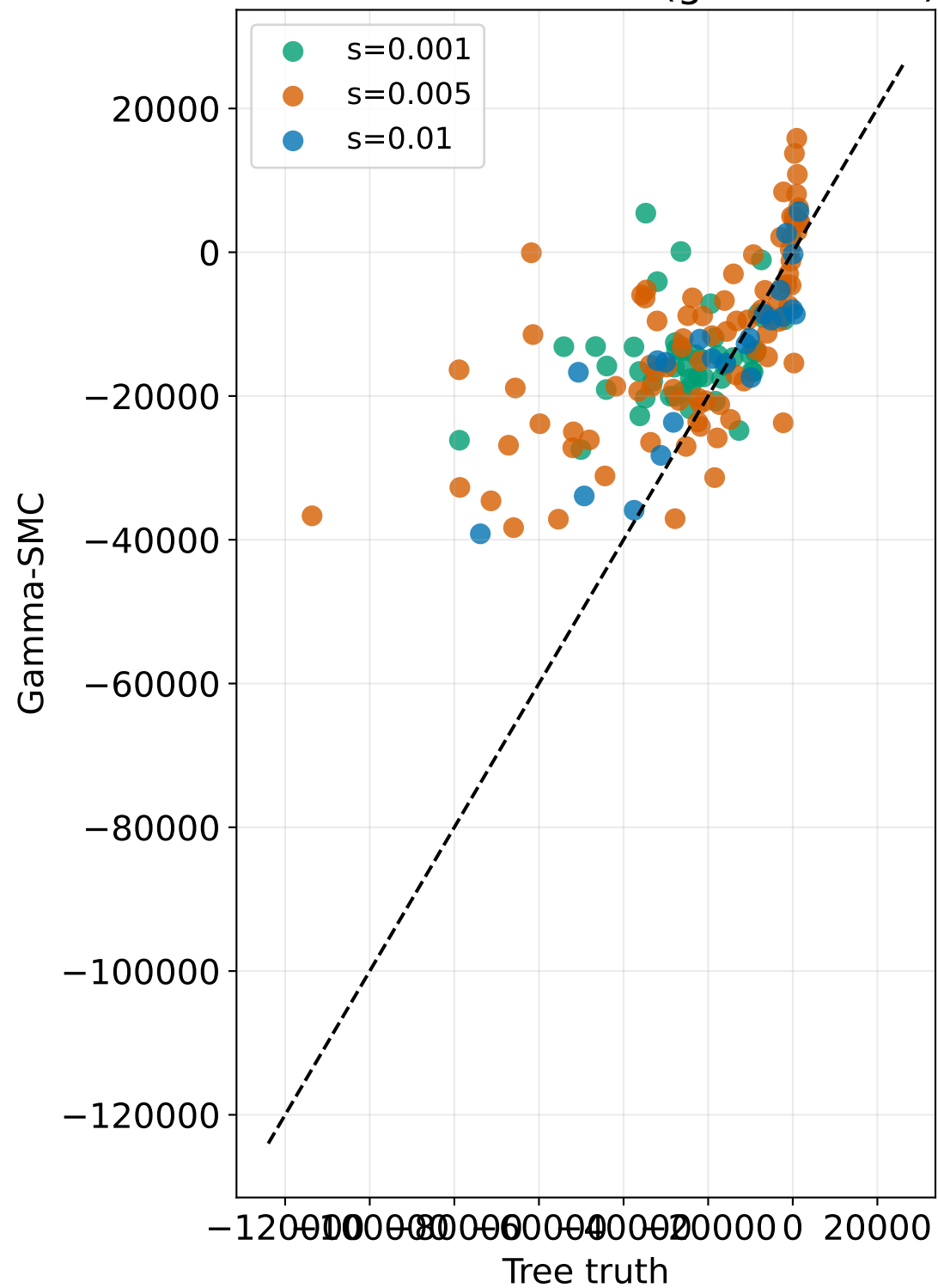
Alt-ref mean TMRCA (generations)
