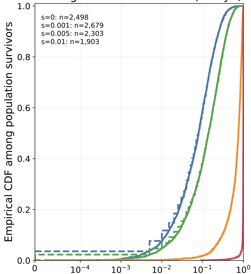
EAS age-matched de novo (50 kya)
