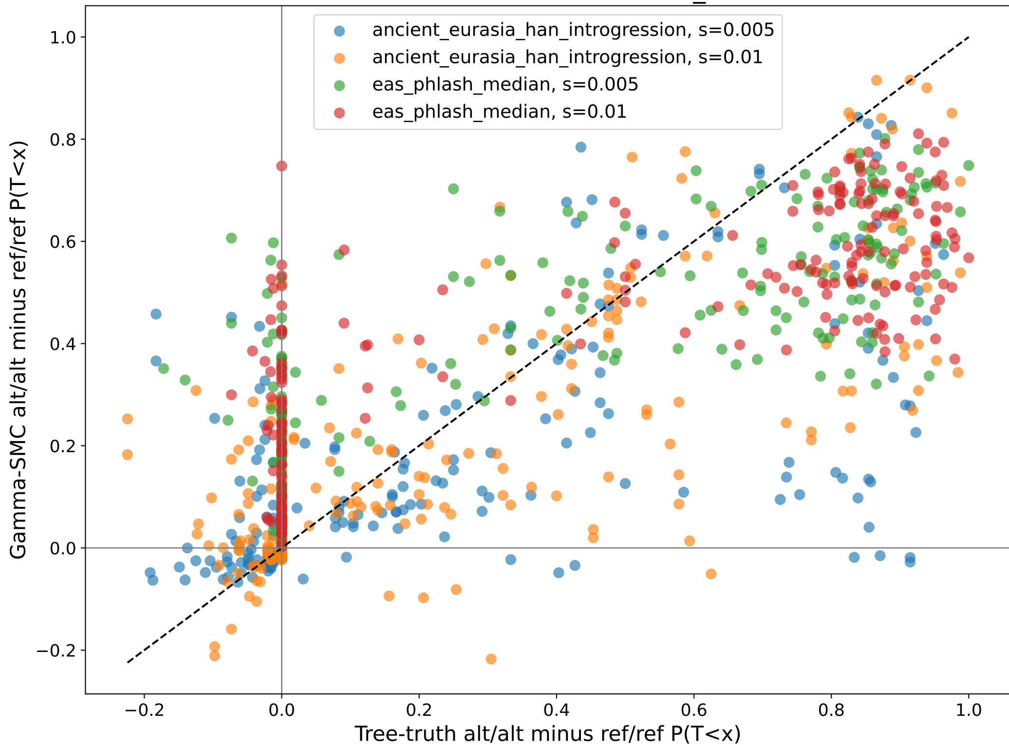
Truth versus Gamma-SMC: focal_nearest
