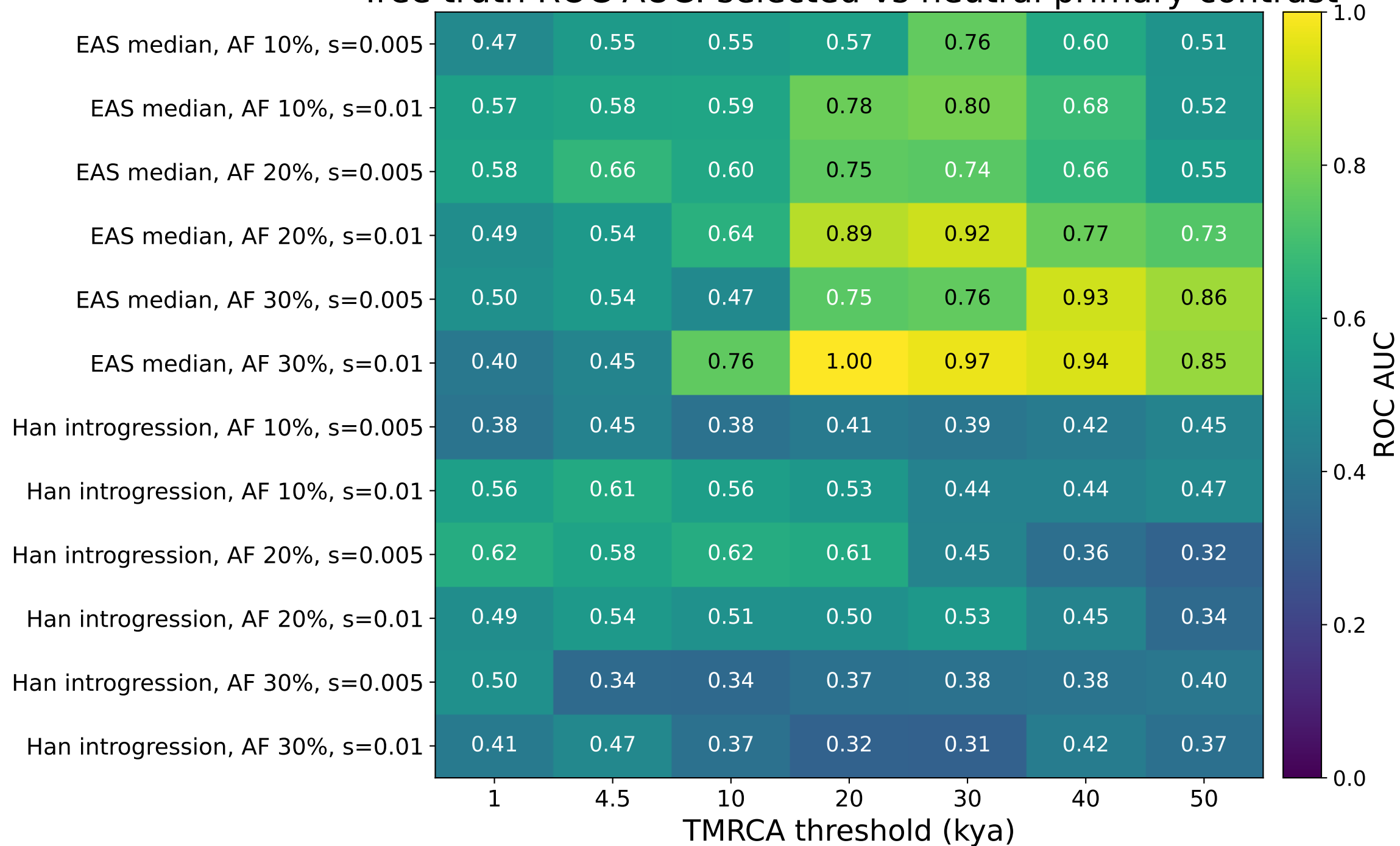
Tree truth ROC AUC: selected vs neutral primary contrast
