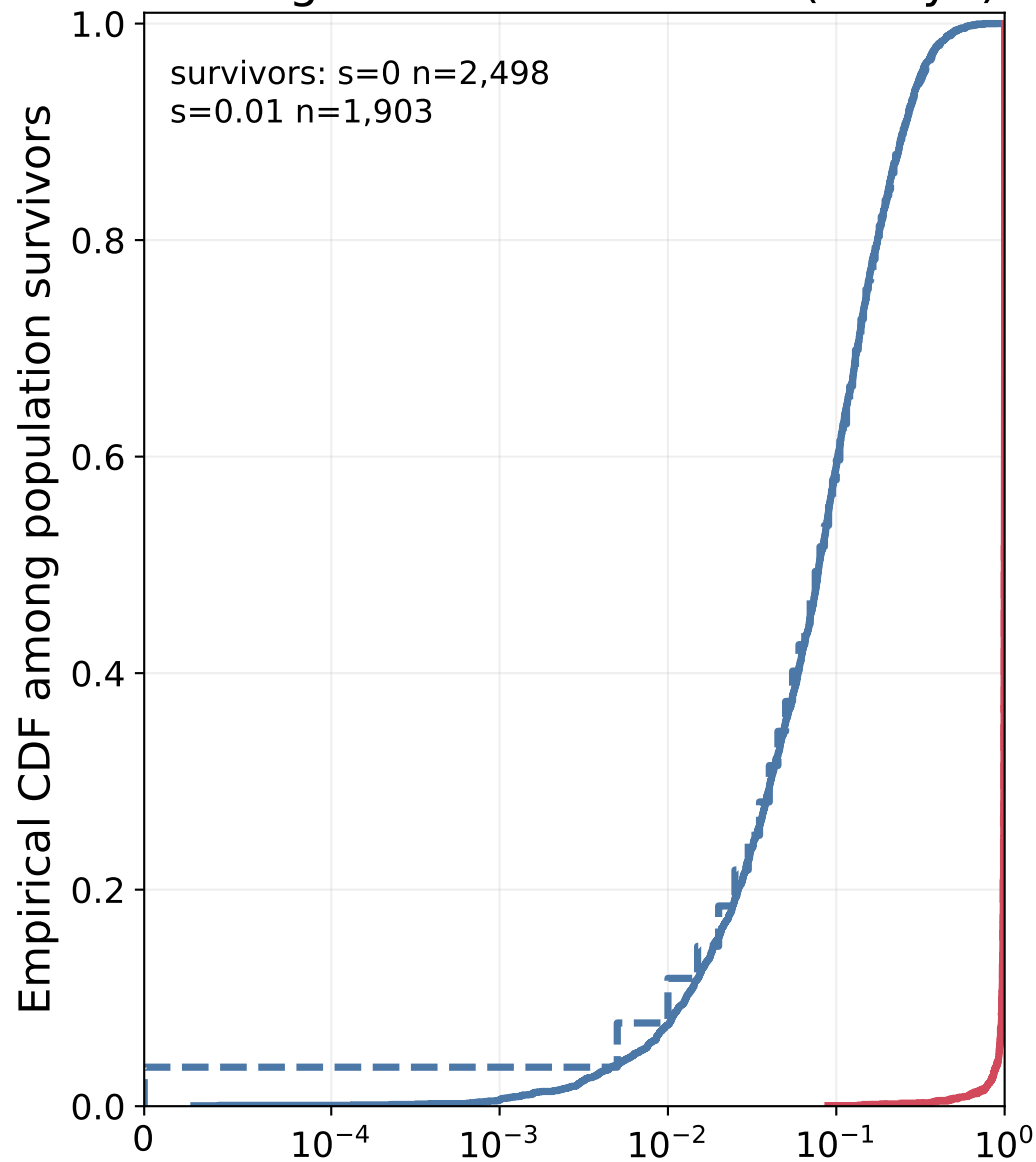
EAS age-matched de novo (50 kya)
