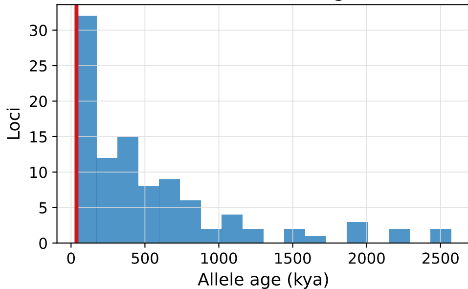
EAS neutral mutation-age draws
