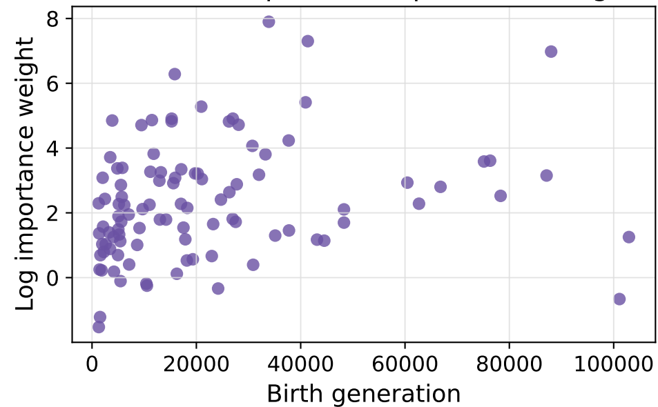
EAS selected-particle importance weights
