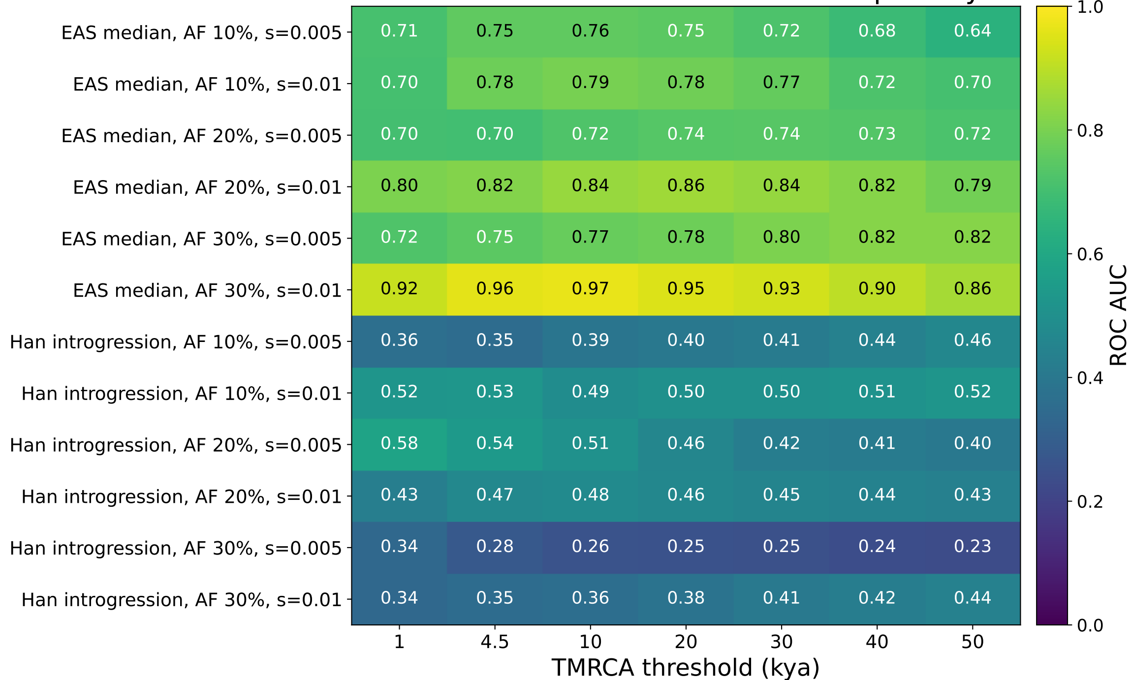
Gamma-SMC ROC AUC: selected vs neutral primary contrast
