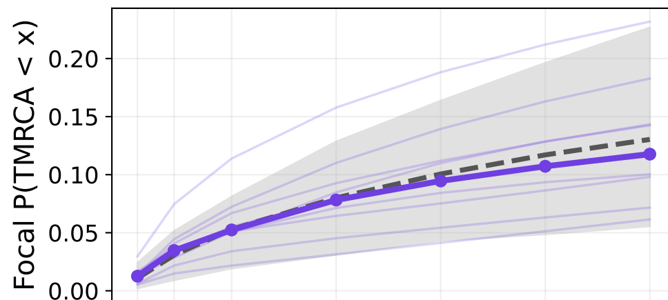
Gamma-SMC
