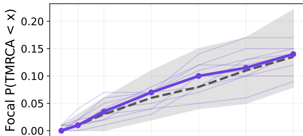
Tree truth
