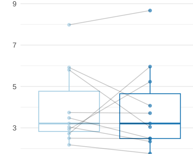
Malic Acid
