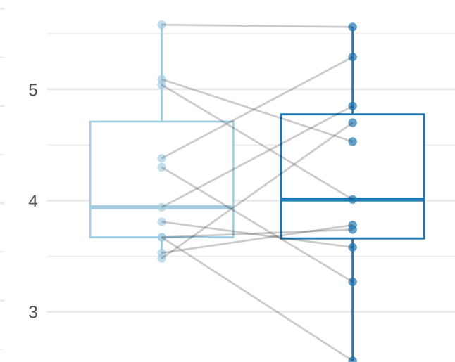
Succinic Acid
