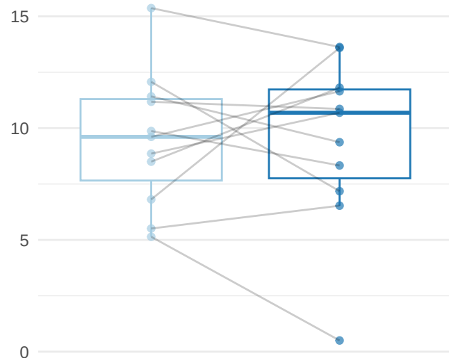
Glucose
