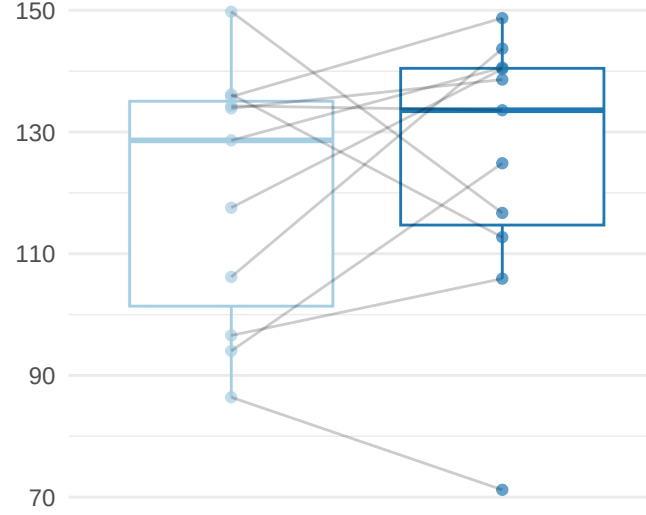
Isocitric Acid
