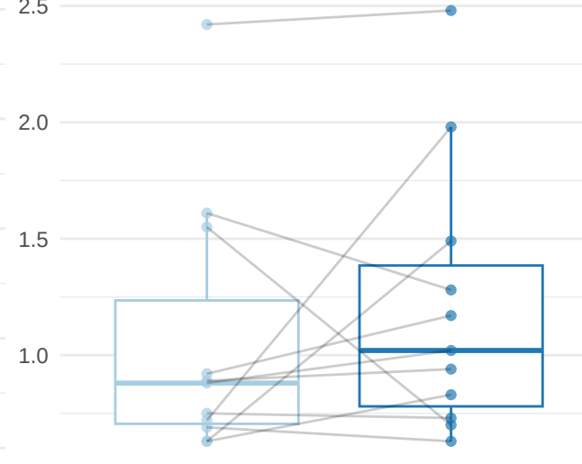
Ketoglutaric Acid
