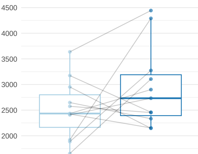
Lactic acid
