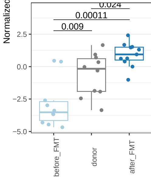
N-methylproline
