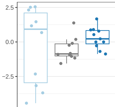
proline
