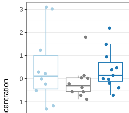
N-methylproline
