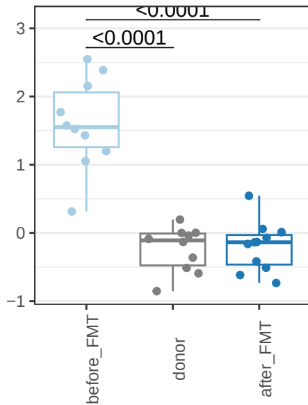
proline
