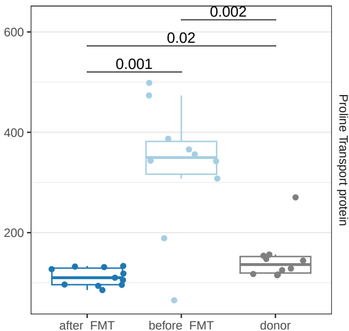
CPM in metagenomics samples
