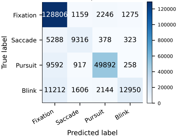
(a) Sample-level
