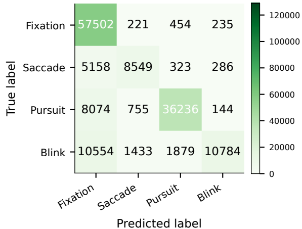
(b) Event-level
